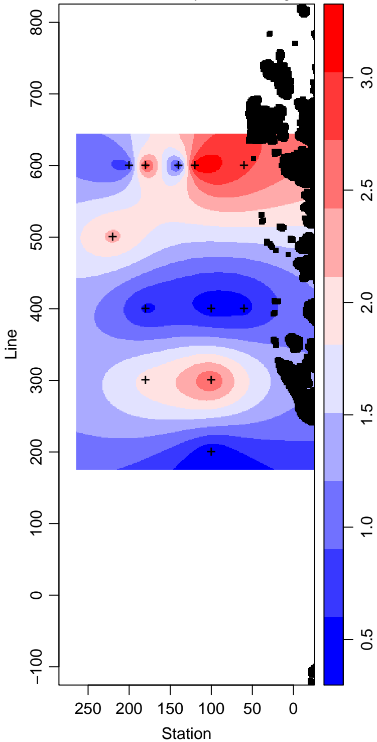
LMG99-01_60_Primary.Production mg m -3
