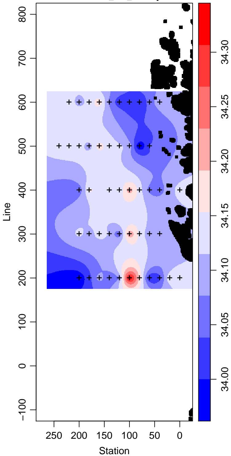
LMG99-01_100_Salinity
