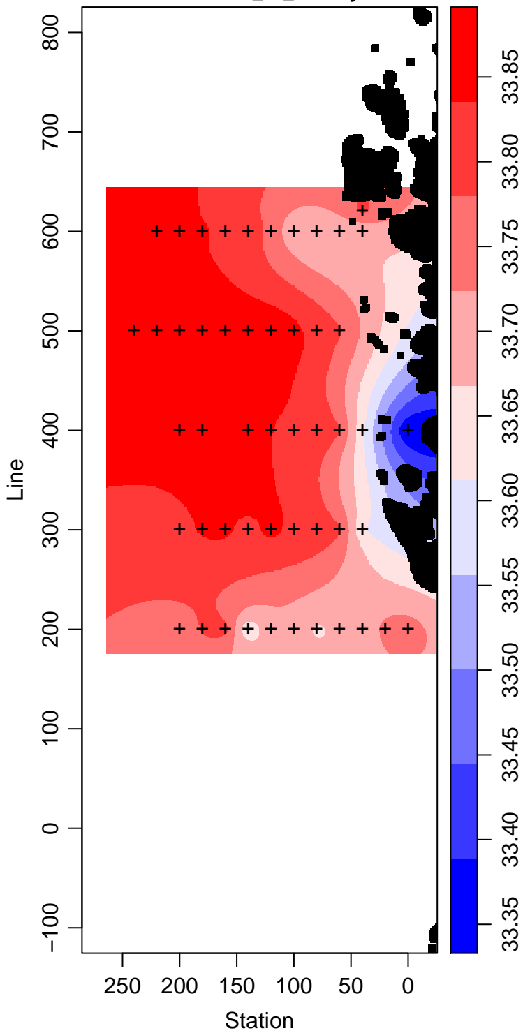
LMG99-01_25_Salinity
