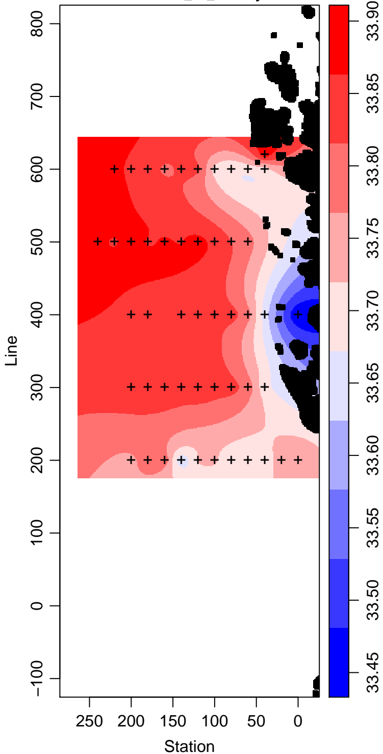
LMG99-01_30_Salinity
