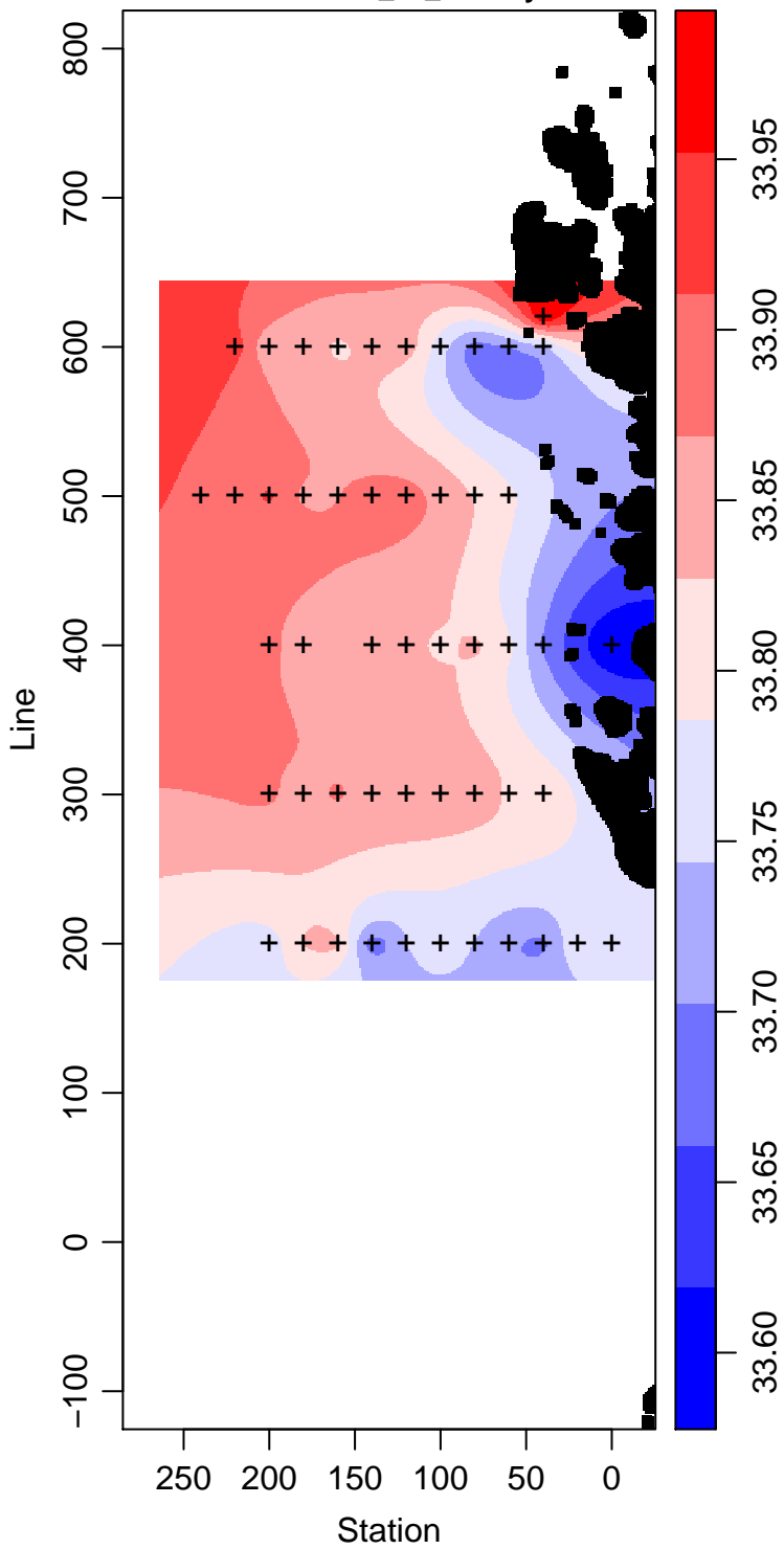
LMG99-01_40_Salinity
