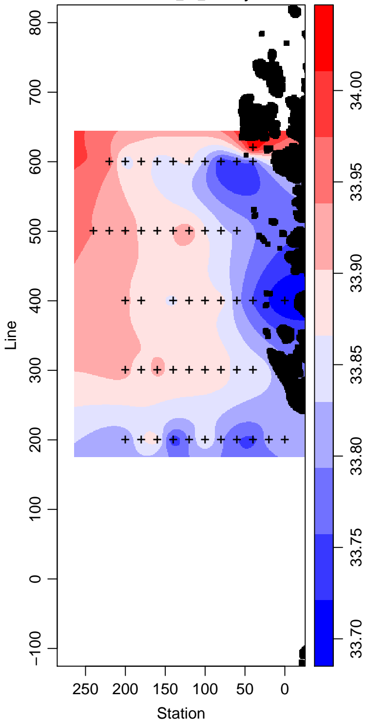
LMG99-01_50_Salinity
