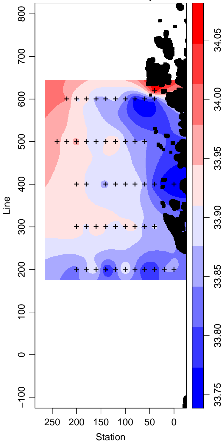
LMG99-01_55_Salinity
