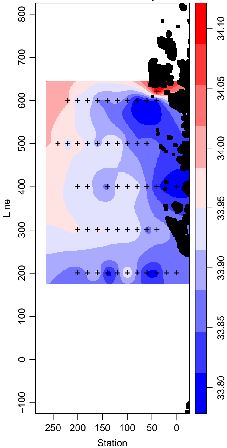
LMG99-01_60_Salinity
