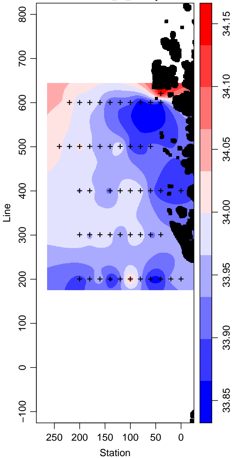
LMG99-01_70_Salinity
