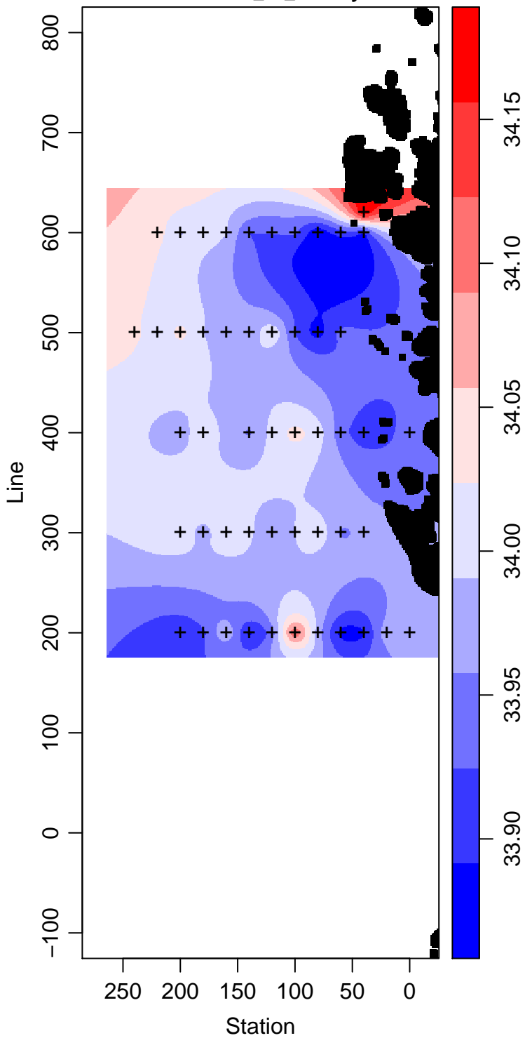
LMG99-01_75_Salinity
