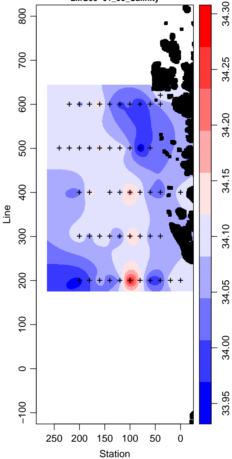
LMG99-01_95_Salinity
