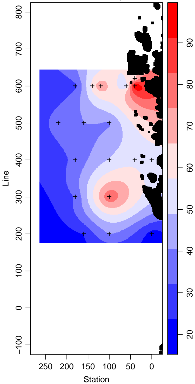
LMG99-01_10_Silicate \mu\text{ mol L}^{-1}
