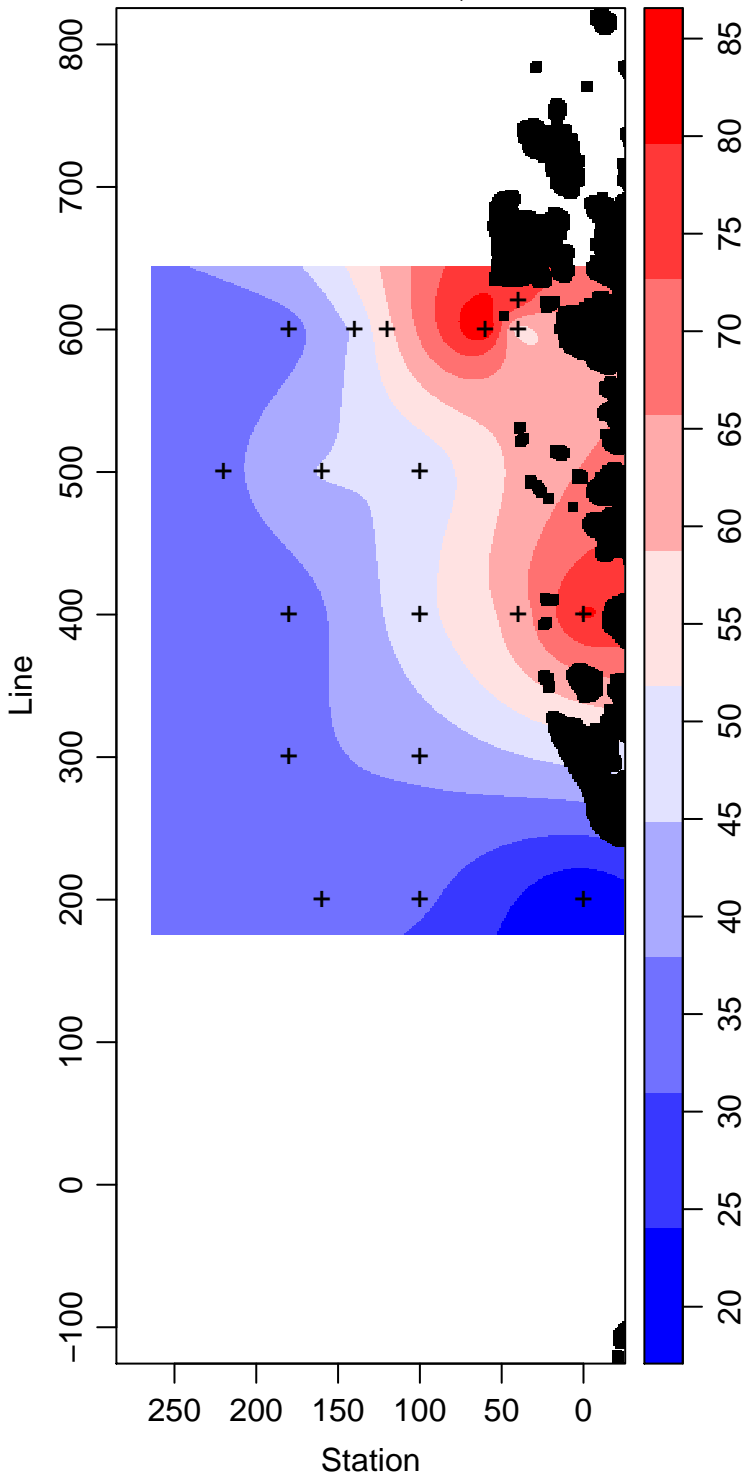
LMG99-01_45_Silicate \mu\text{ mol L}^{-1}
