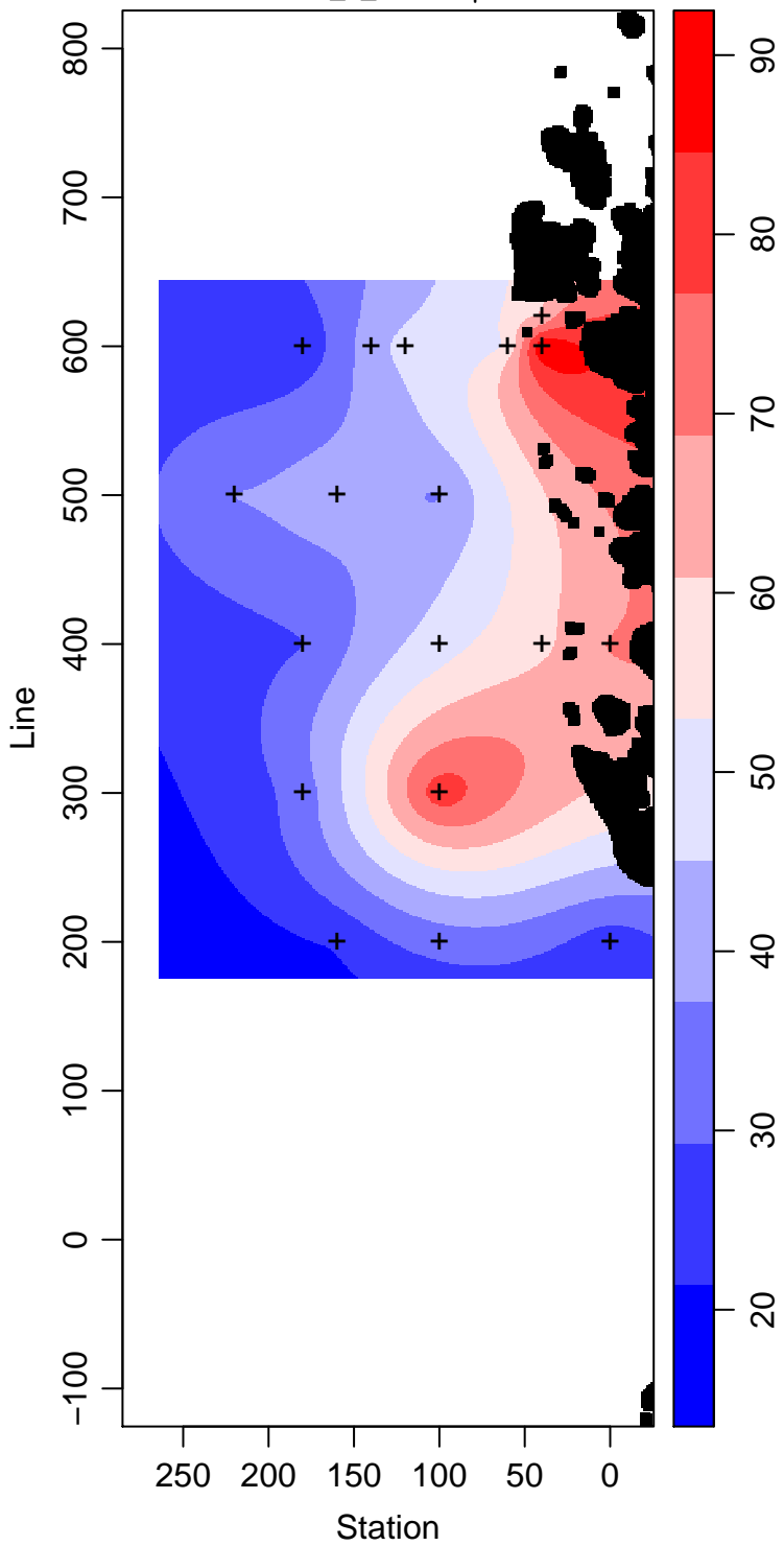
LMG99-01_5_Silicate \mu\text{ mol L}^{-1}
