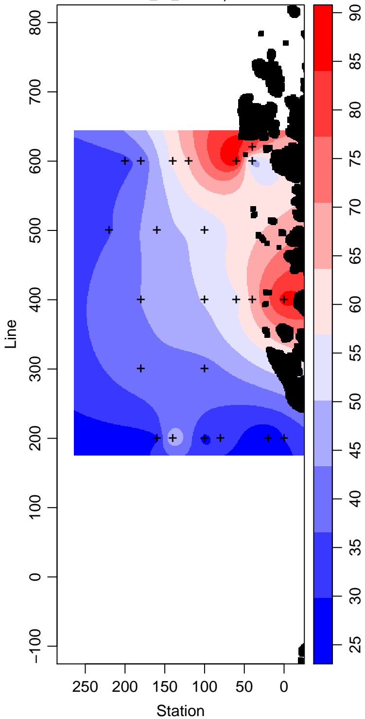
LMG99-01_60_Silicate \mu\text{ mol L}^{-1}
