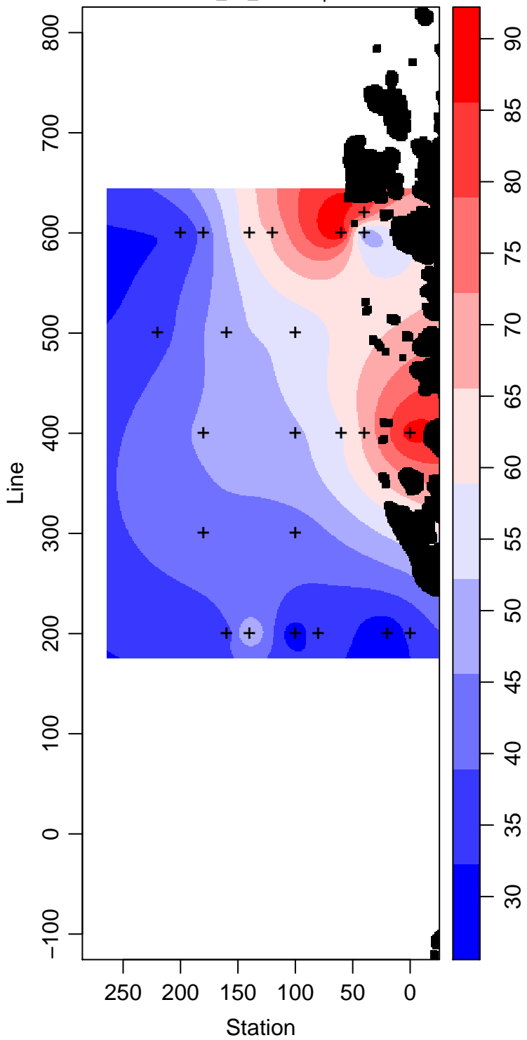
LMG99-01_65_Silicate \mu\text{ mol L}^{-1}
