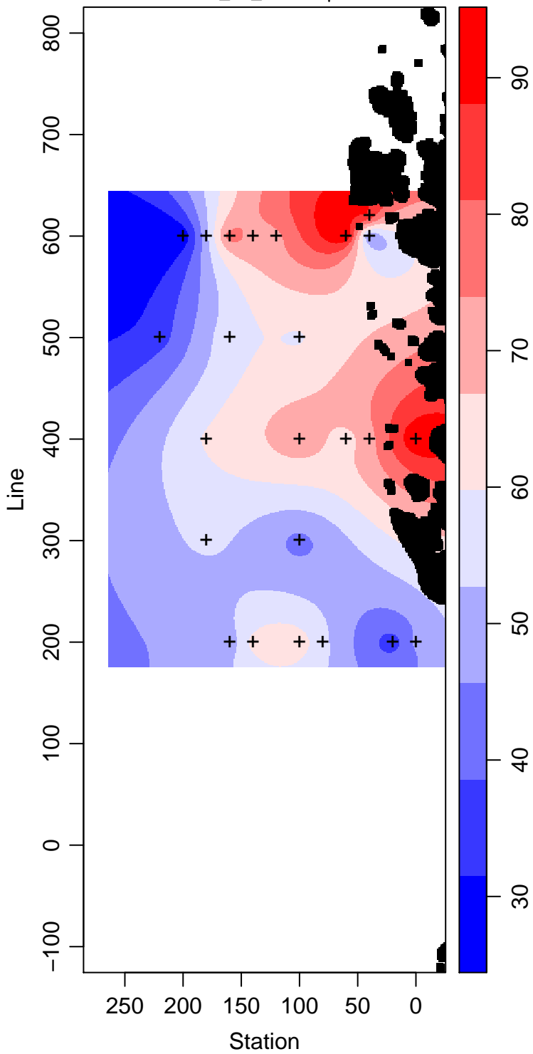
LMG99-01_80_Silicate \mu\text{ mol L}^{-1}
