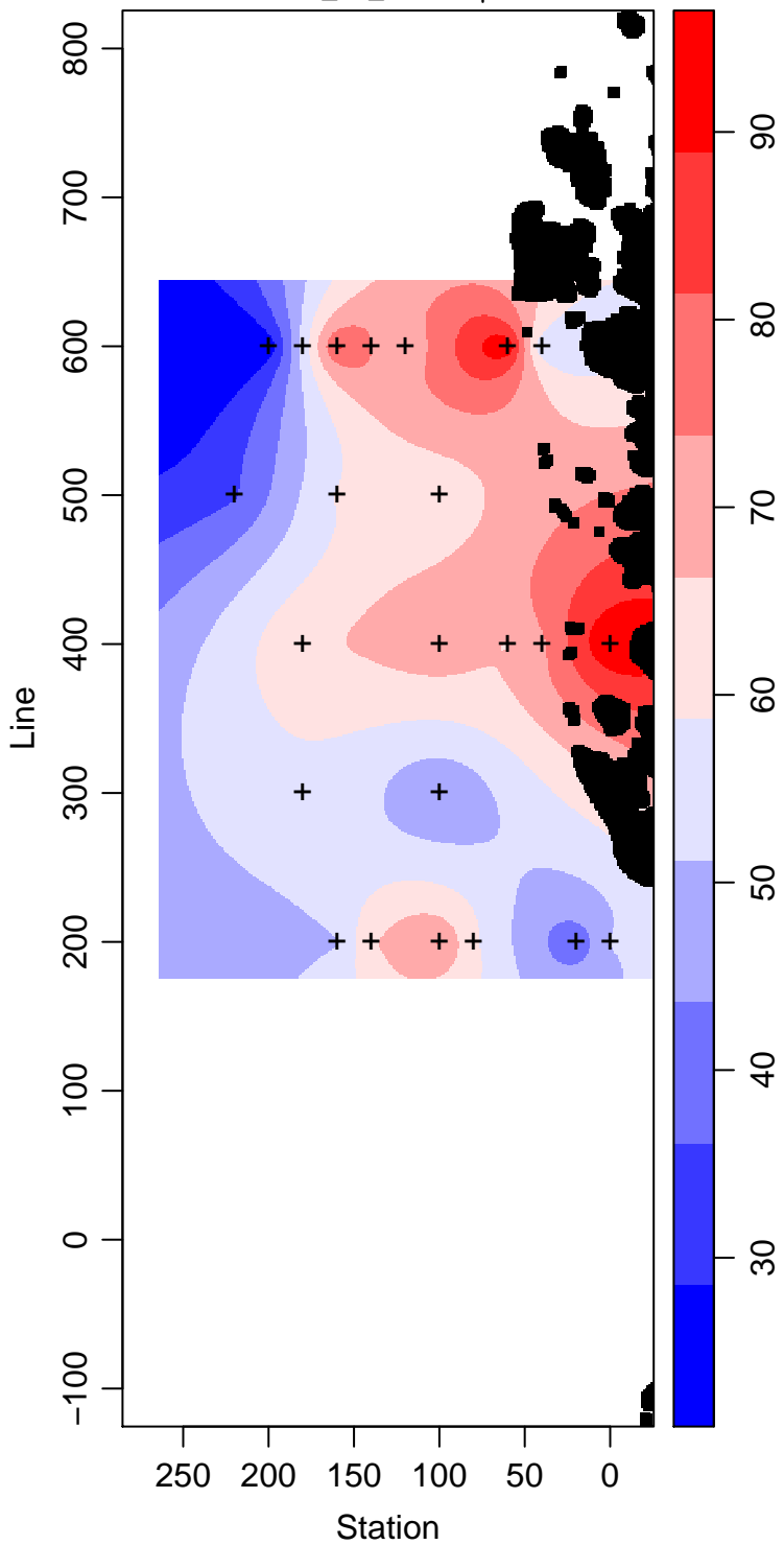
LMG99-01_85_Silicate \mu\text{ mol L}^{-1}
