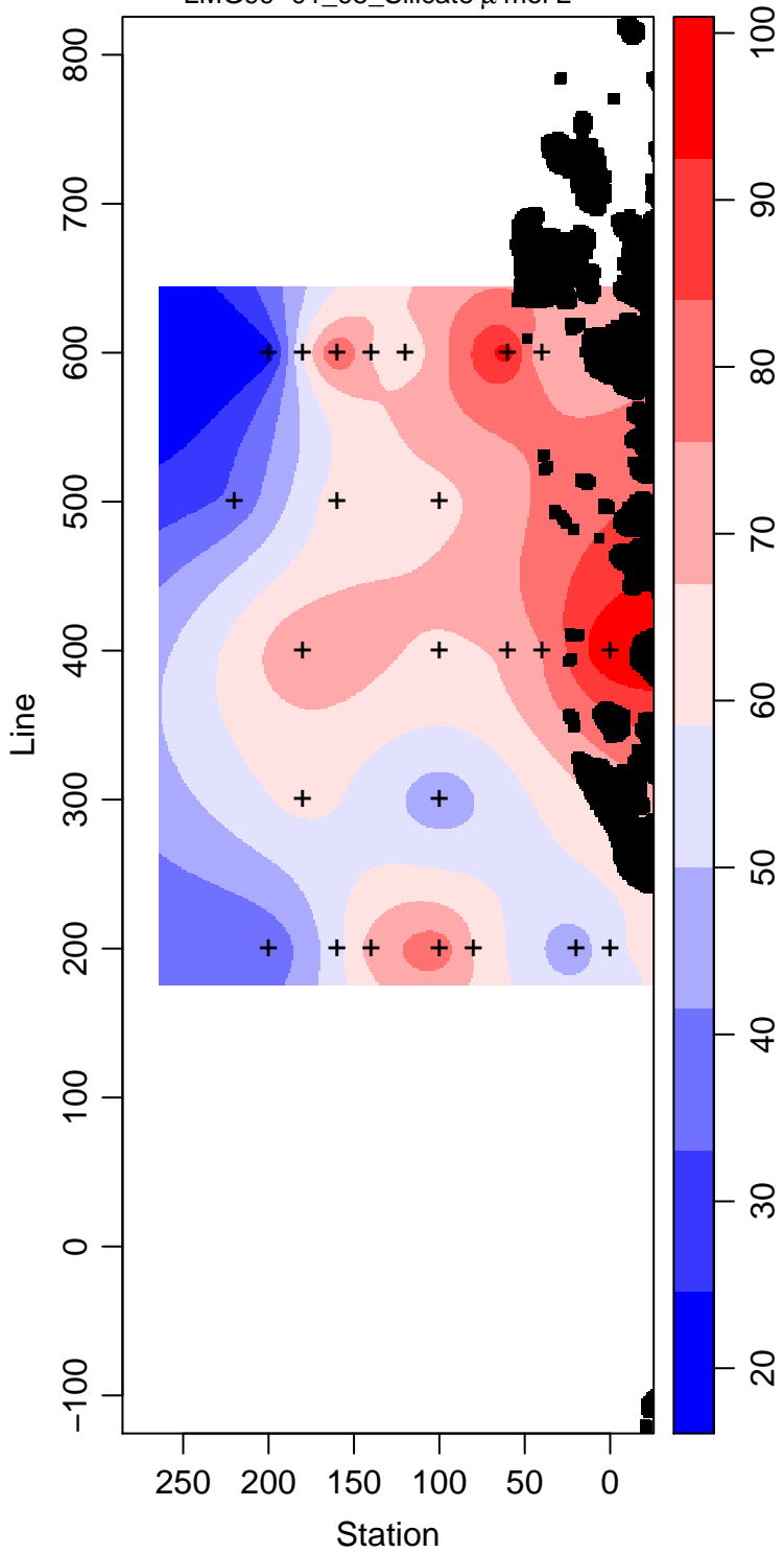
LMG99-01_95_Silicate \mu\text{ mol L}^{-1}
