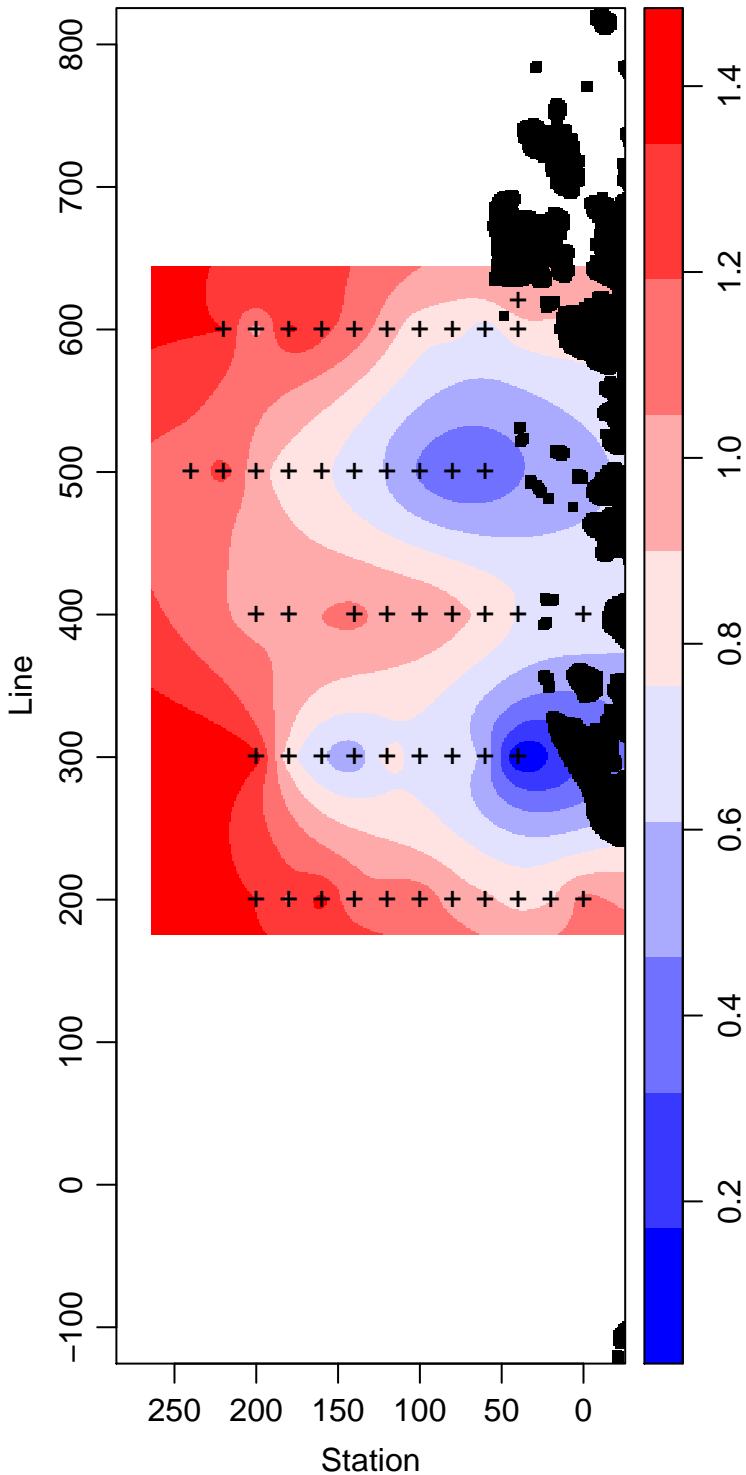
LMG99-01_1_Temperature ° Celsius
