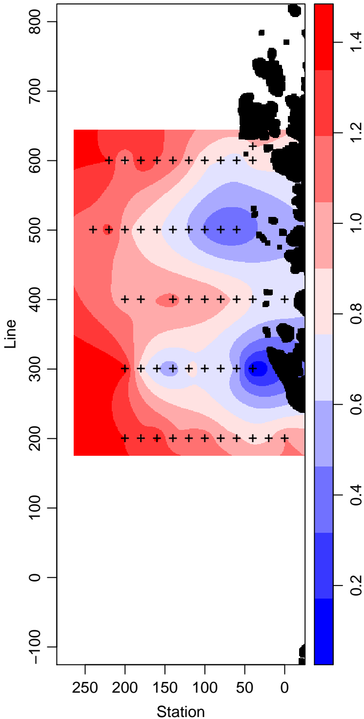
LMG99-01_5_Temperature ° Celsius
