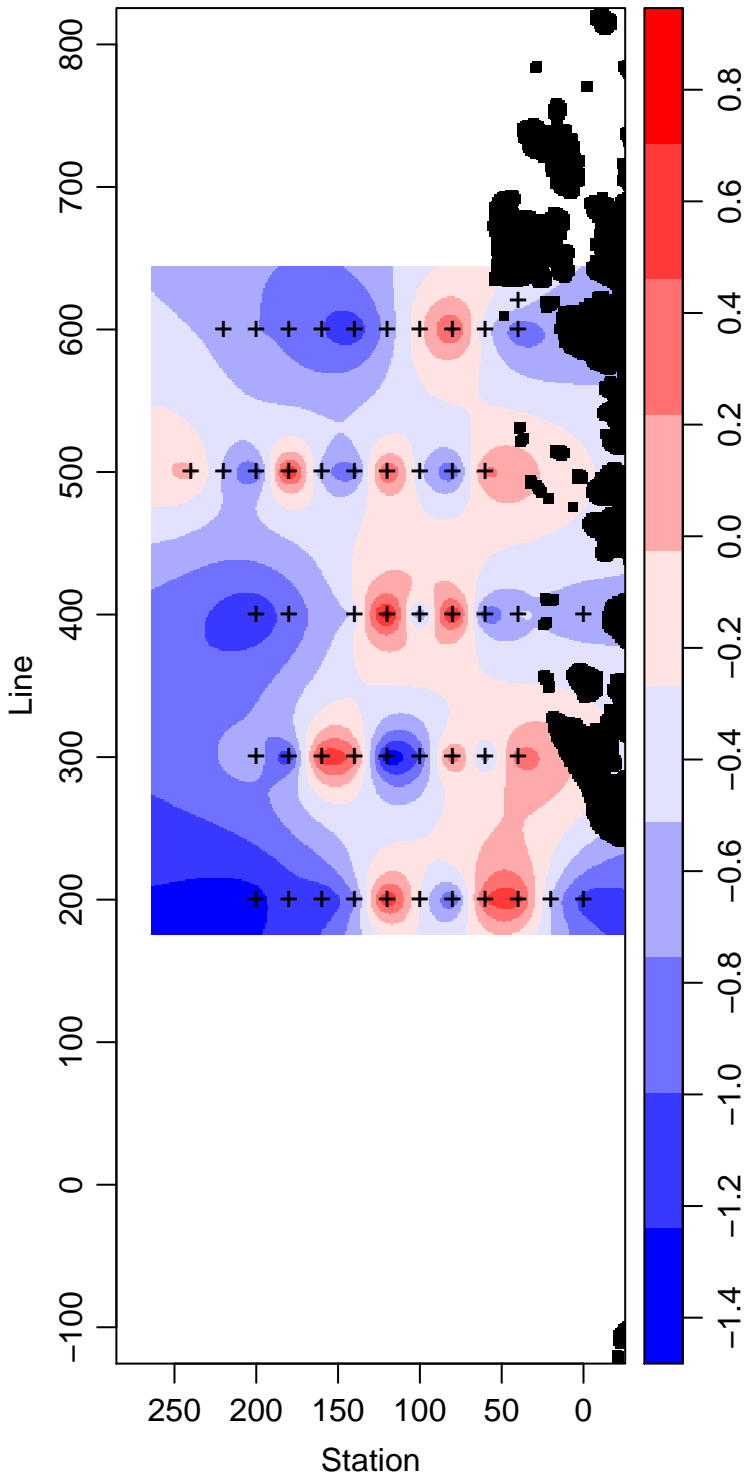
LMG99-01_90_Temperature ° Celsius
