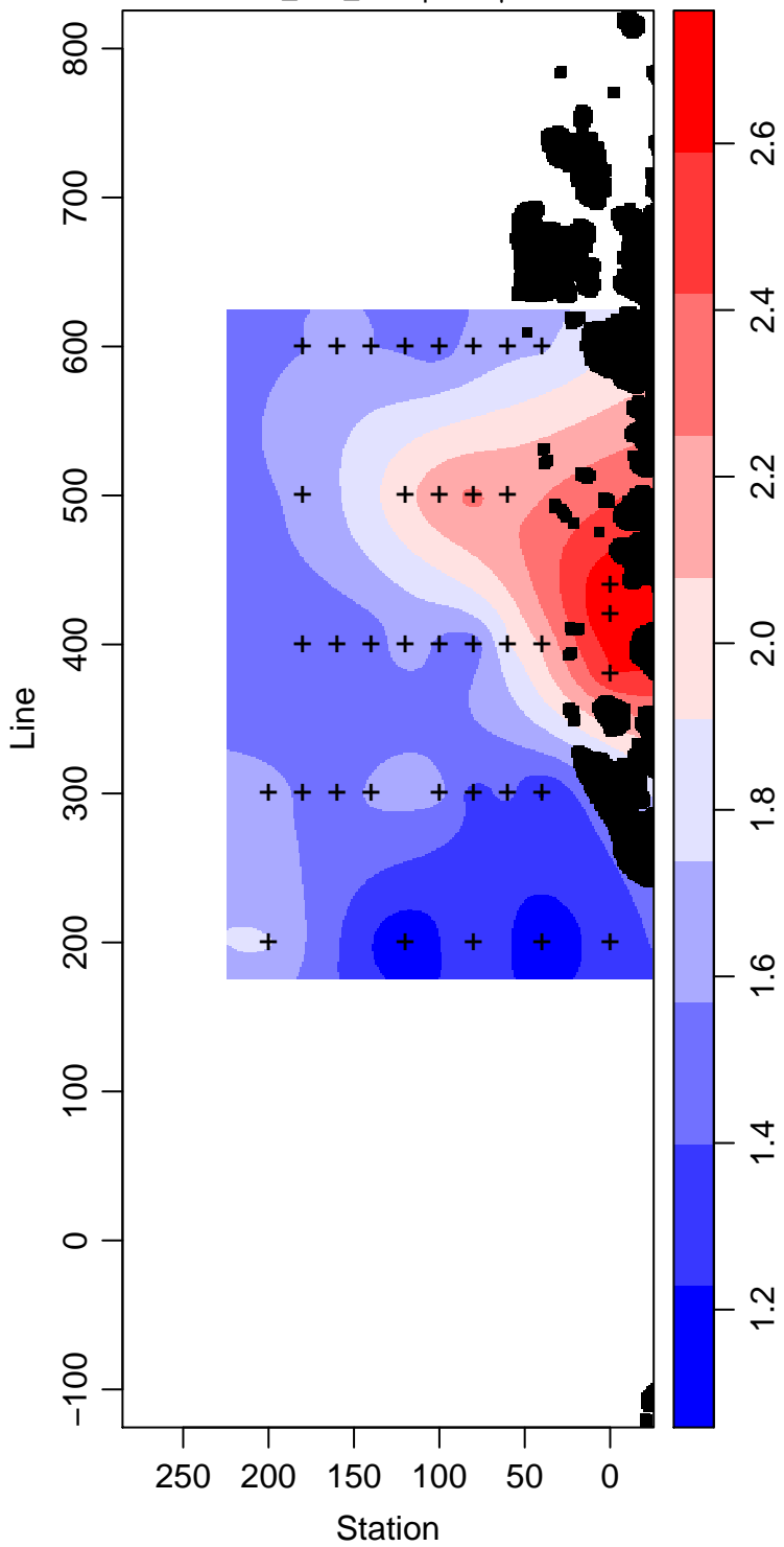
PD93-01_100_Phosphate \mu\text{ mol L}^{-1}
