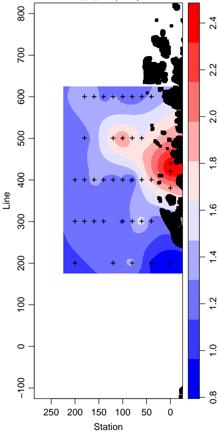
PD93-01_20_Phosphate \mu\text{ mol L}^{-1}
