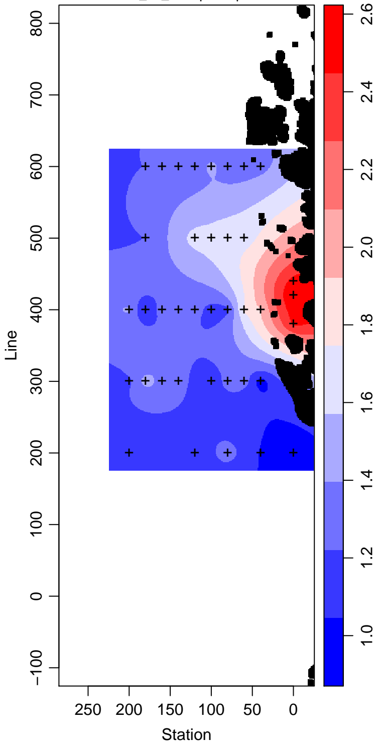
PD93-01_35_Phosphate \mu\text{ mol L}^{-1}
