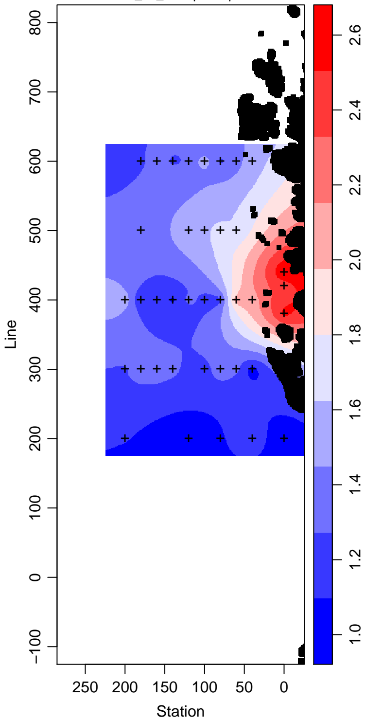
PD93-01_45_Phosphate \mu\text{ mol L}^{-1}
