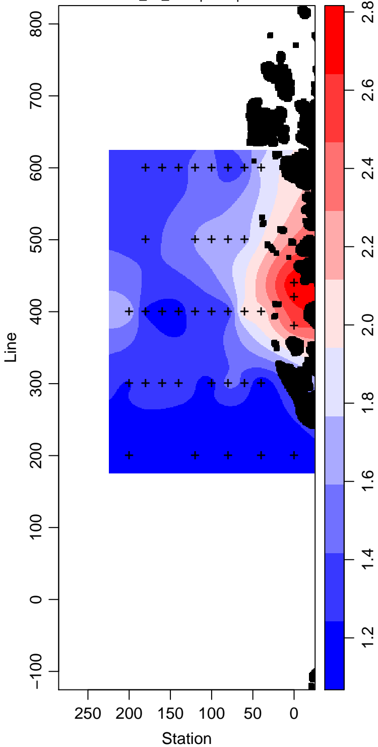
PD93-01_55_Phosphate \mu\text{ mol L}^{-1}
