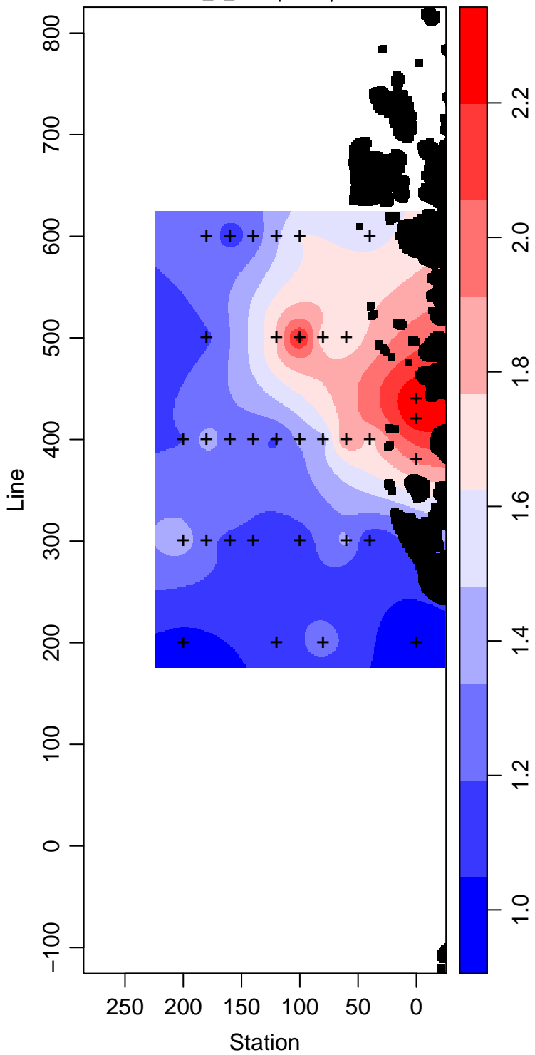
PD93-01_5_Phosphate \mu\text{ mol L}^{-1}
