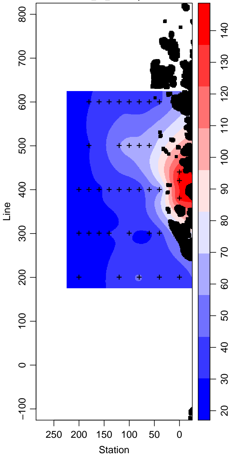
PD93-01_15_Silicate \mu\text{ mol L}^{-1}
