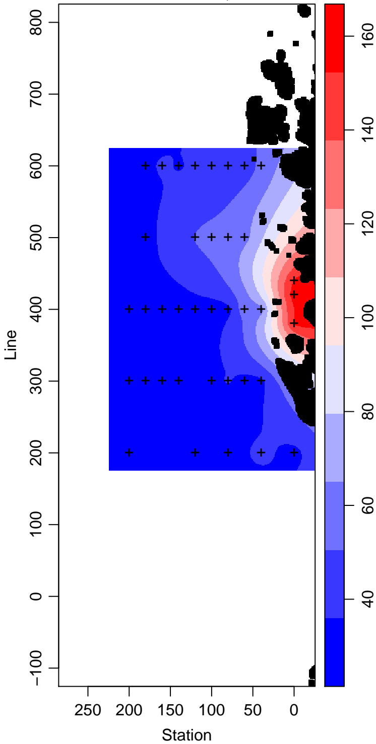
PD93-01_45_Silicate \mu\text{ mol L}^{-1}
