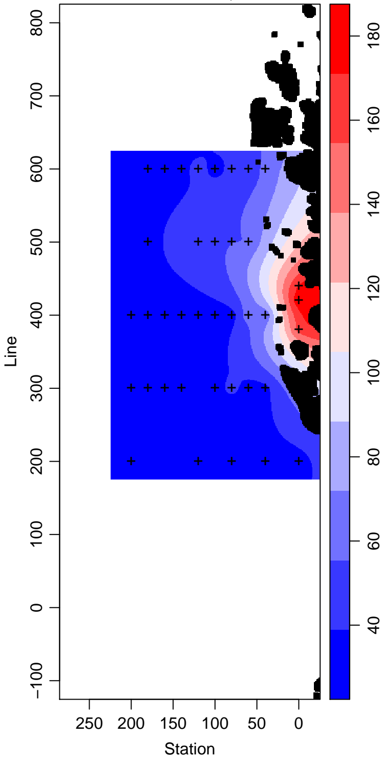
PD93-01_50_Silicate \mu\text{ mol L}^{-1}
