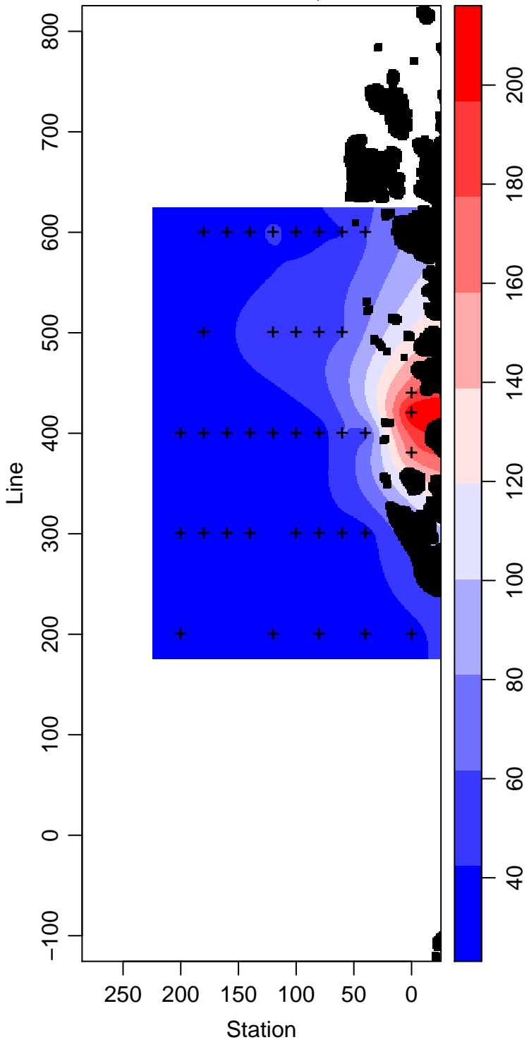
PD93-01_55_Silicate \mu\text{ mol L}^{-1}
