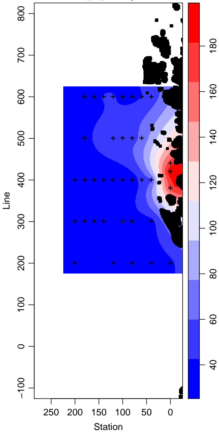
PD93-01_70_Silicate \mu\text{ mol L}^{-1}
