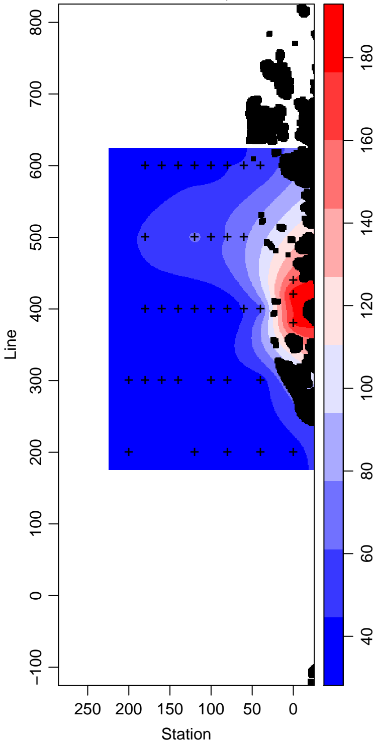
PD93-01_95_Silicate \mu\text{ mol L}^{-1}
