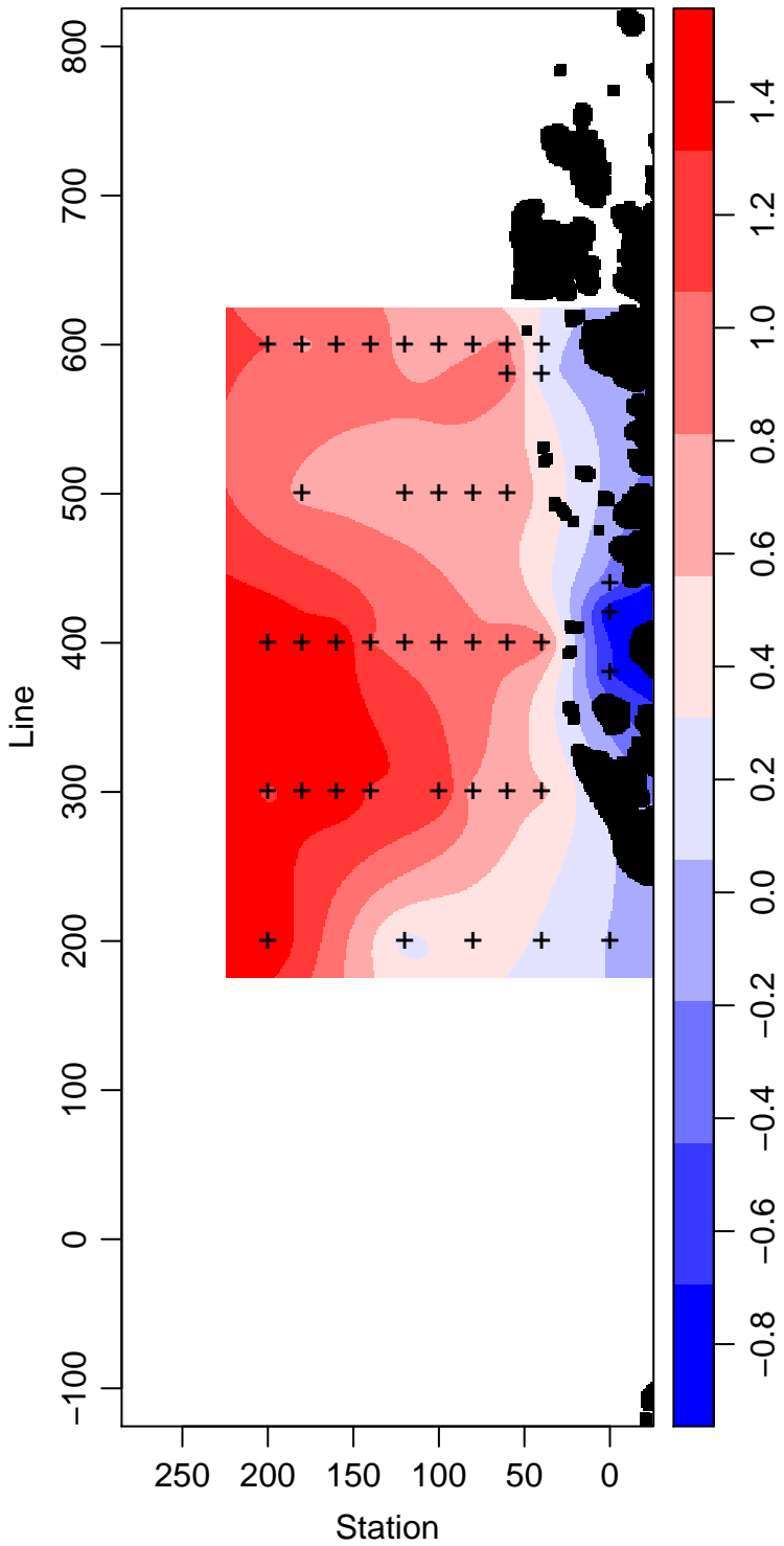
PD93-01_20_Temperature ° Celsius
