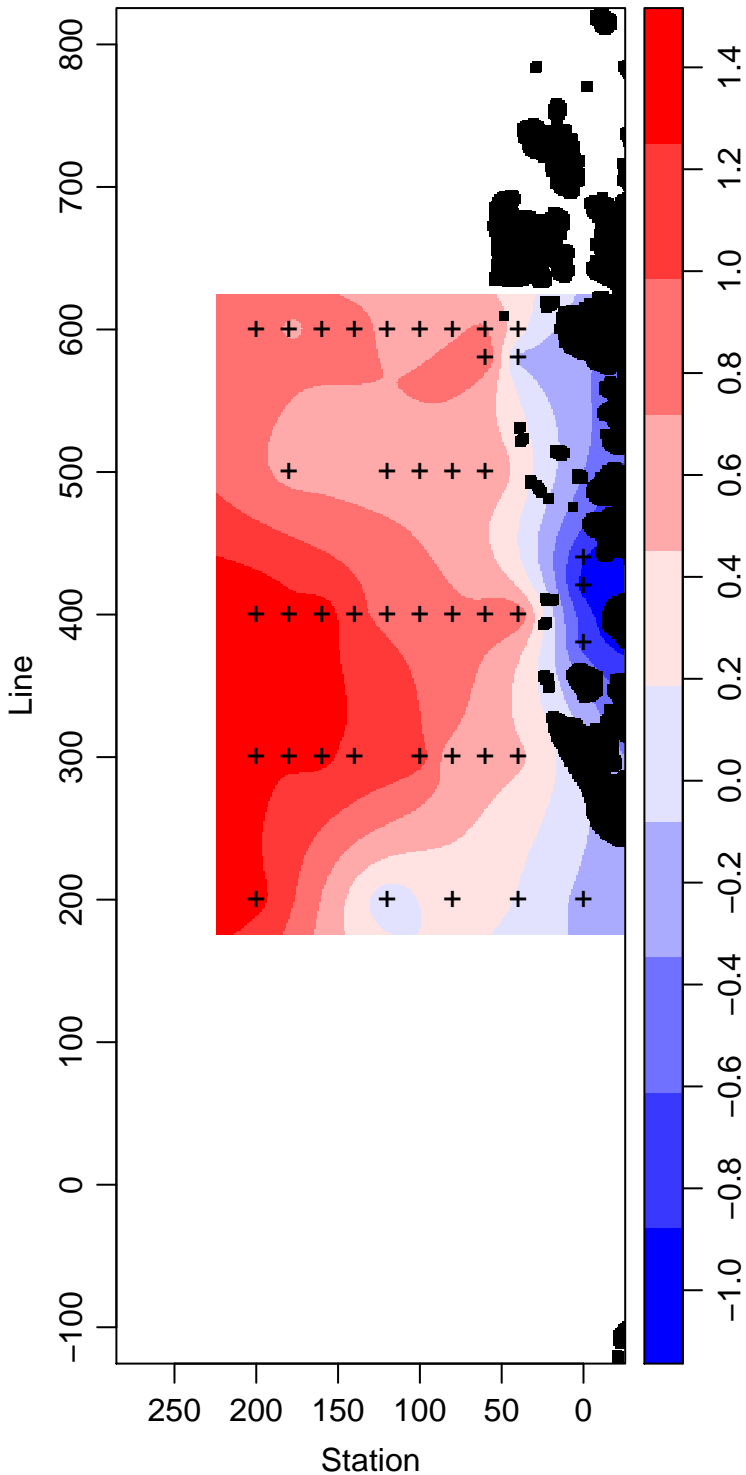
PD93-01_25_Temperature ° Celsius
