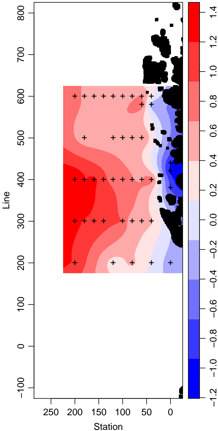
PD93-01_30_Temperature ° Celsius
