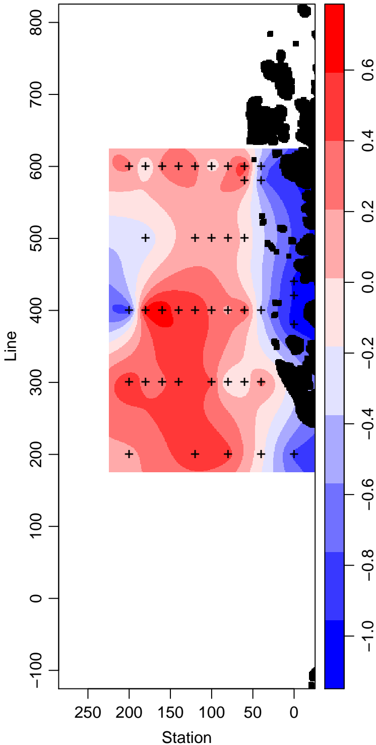
PD93-01_60_Temperature ° Celsius
