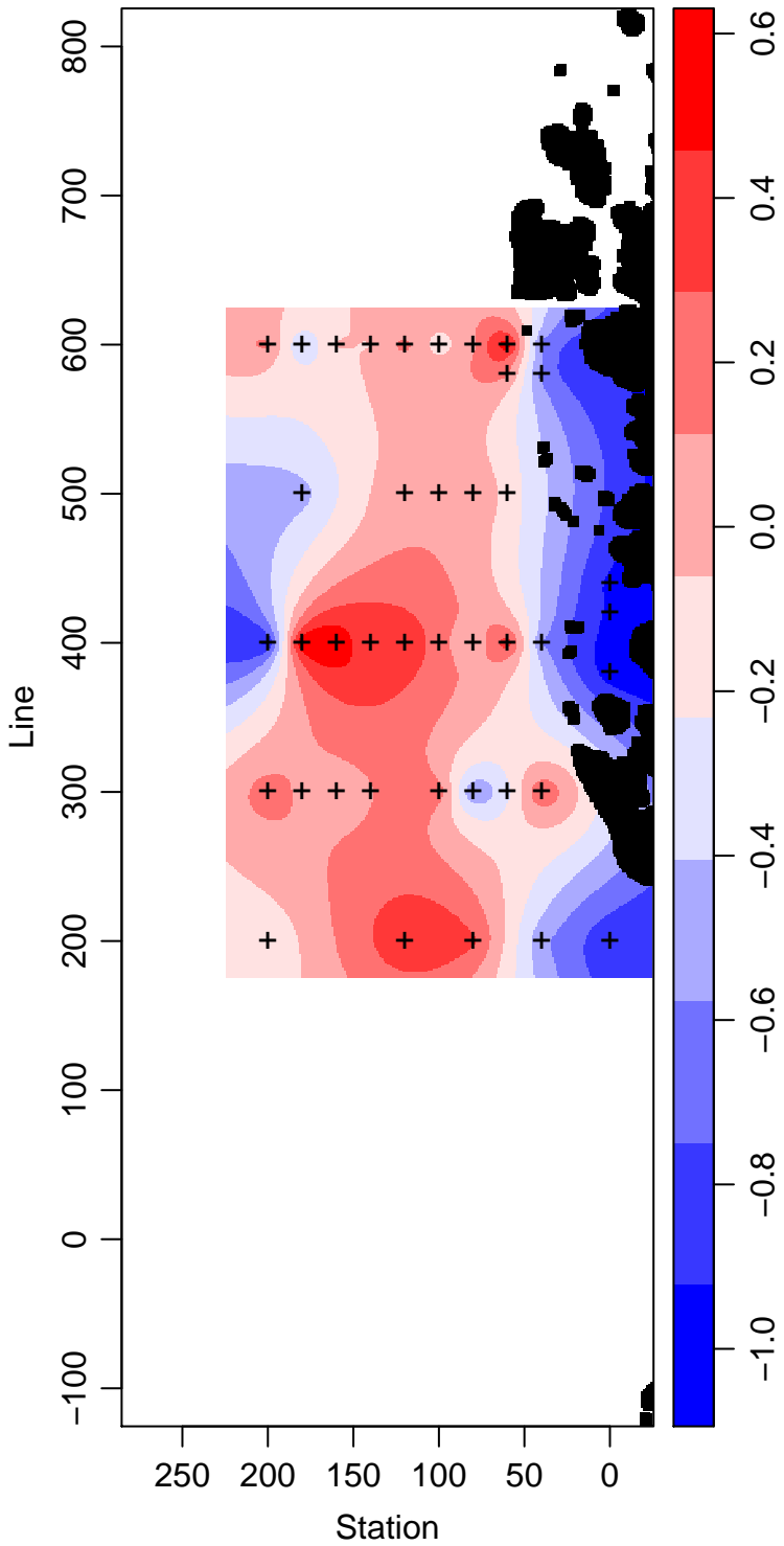
PD93-01_65_Temperature ° Celsius
