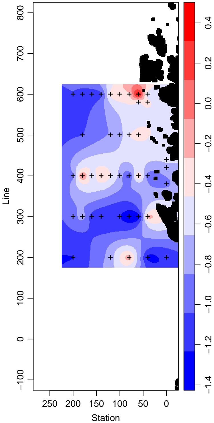
PD93-01_85_Temperature ° Celsius
