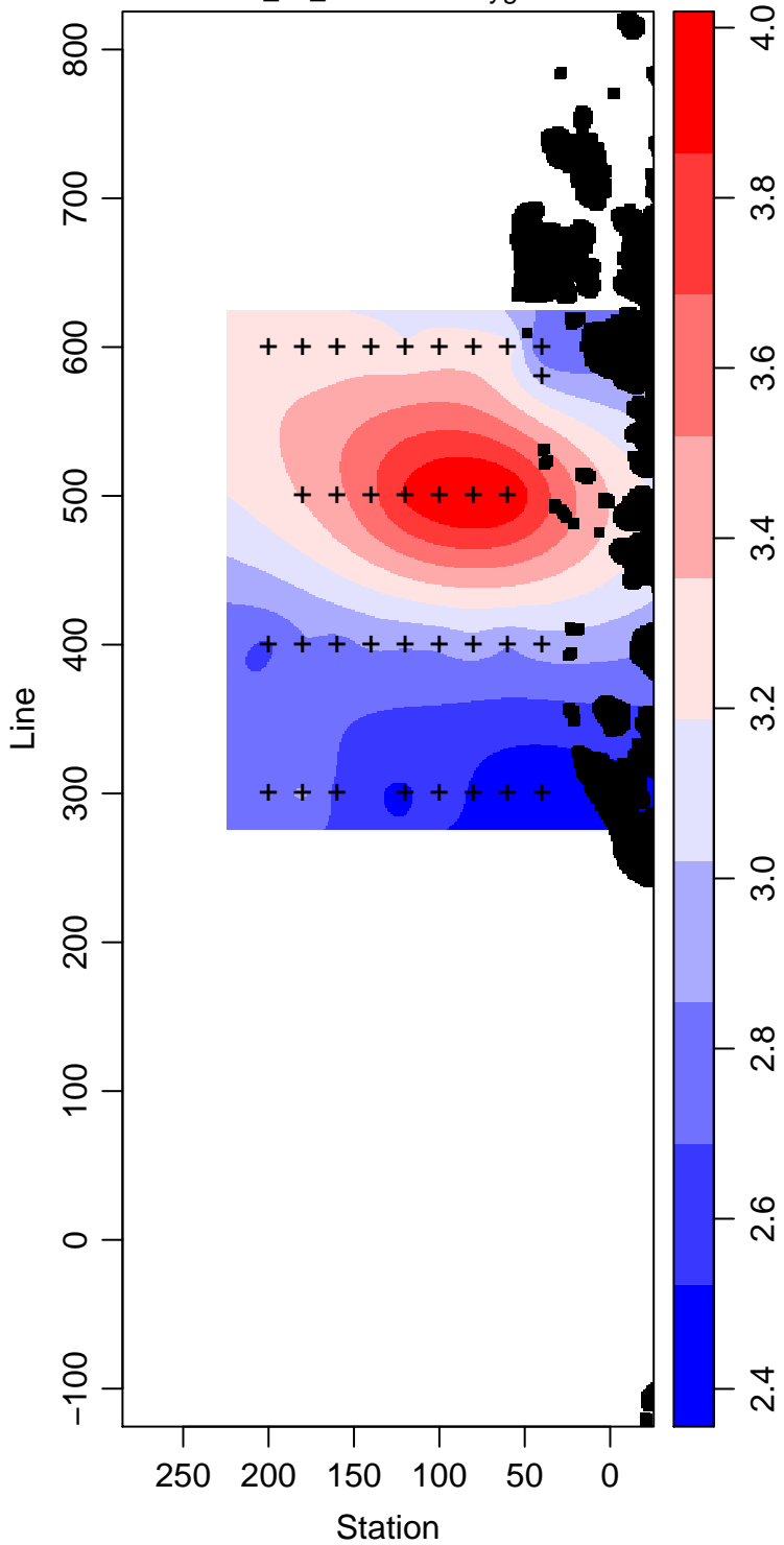
PD94-01_10_Dissolved.Oxygen ml L -1
