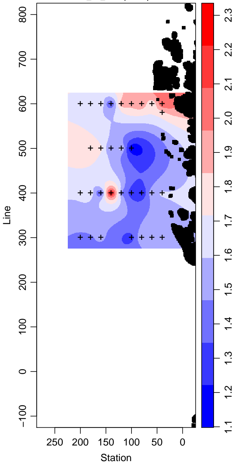
PD94-01_10_Phosphate \mu\text{ mol L}^{-1}
