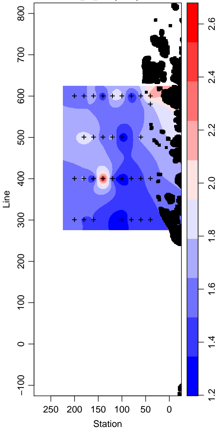
PD94-01_15_Phosphate \mu\text{ mol L}^{-1}
