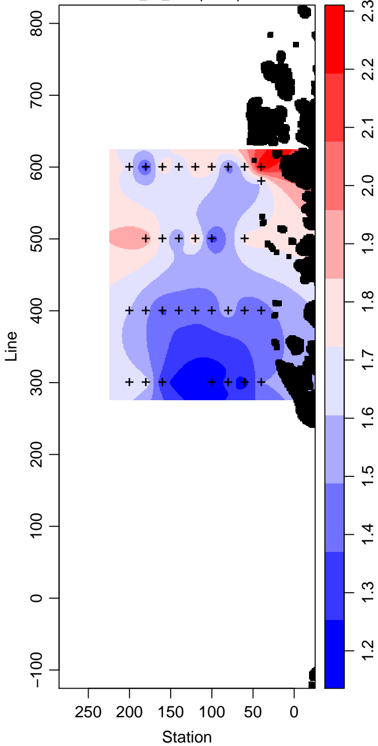
PD94-01_25_Phosphate \mu\text{ mol L}^{-1}
