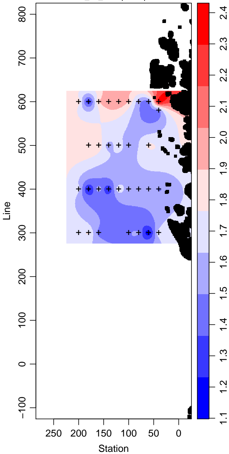
PD94-01_40_Phosphate \mu\text{ mol L}^{-1}
