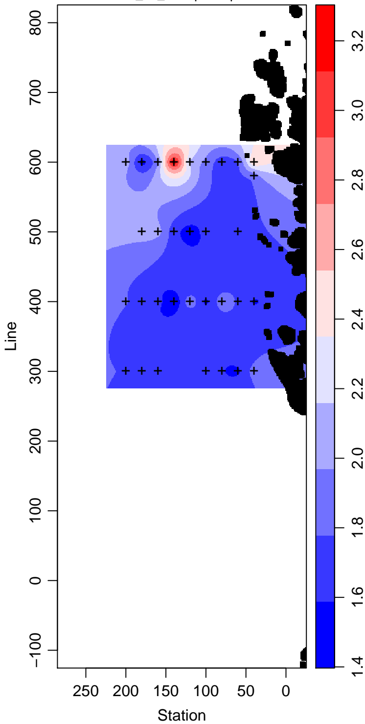
PD94-01_55_Phosphate \mu\text{ mol L}^{-1}
