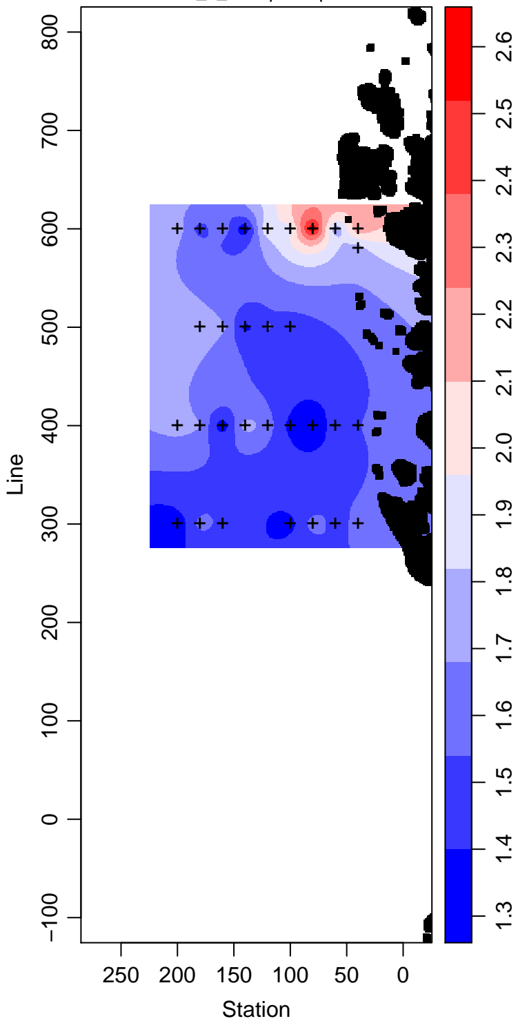
PD94-01_5_Phosphate \mu\text{ mol L}^{-1}
