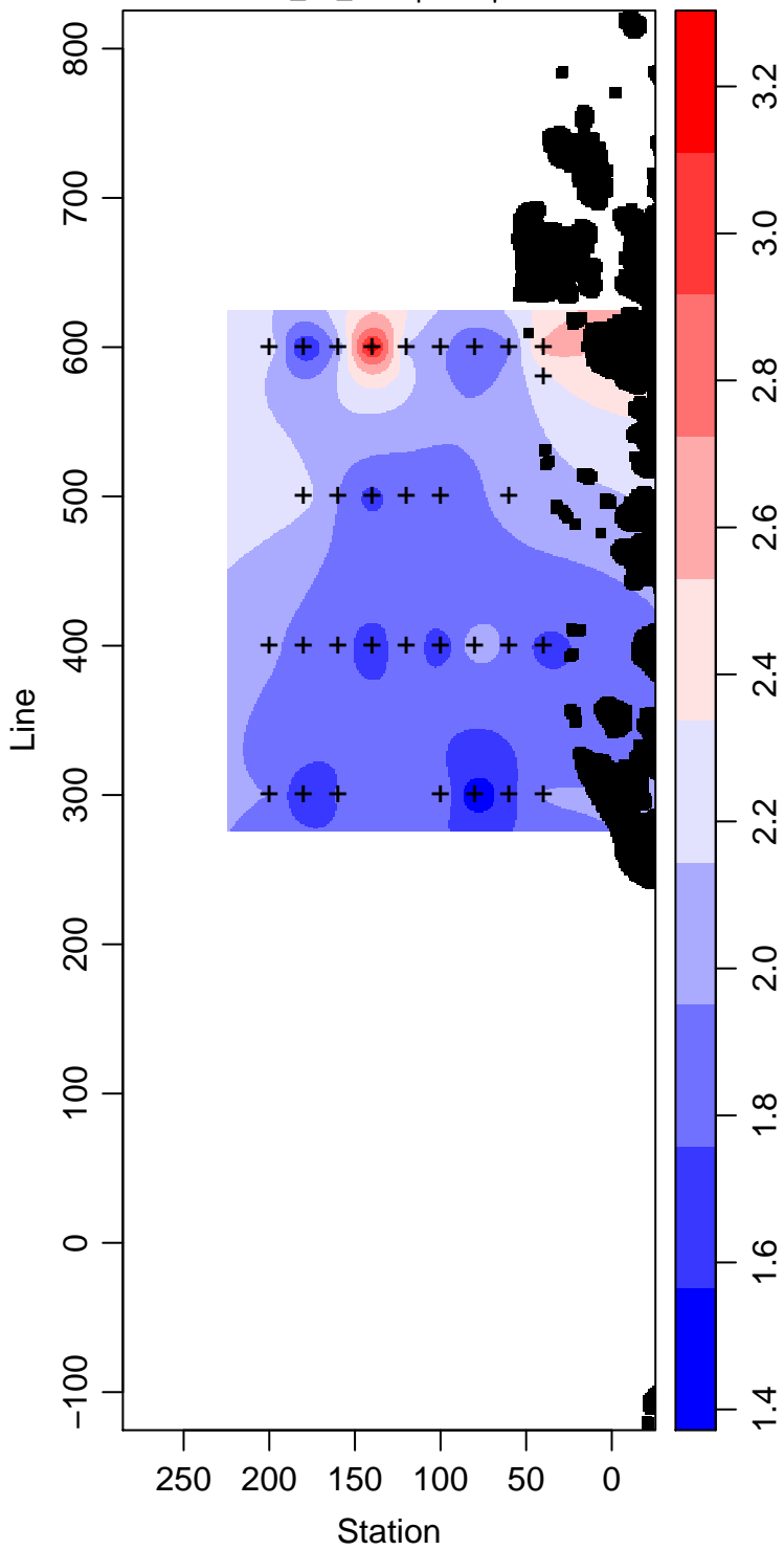
PD94-01_70_Phosphate \mu\text{ mol L}^{-1}
