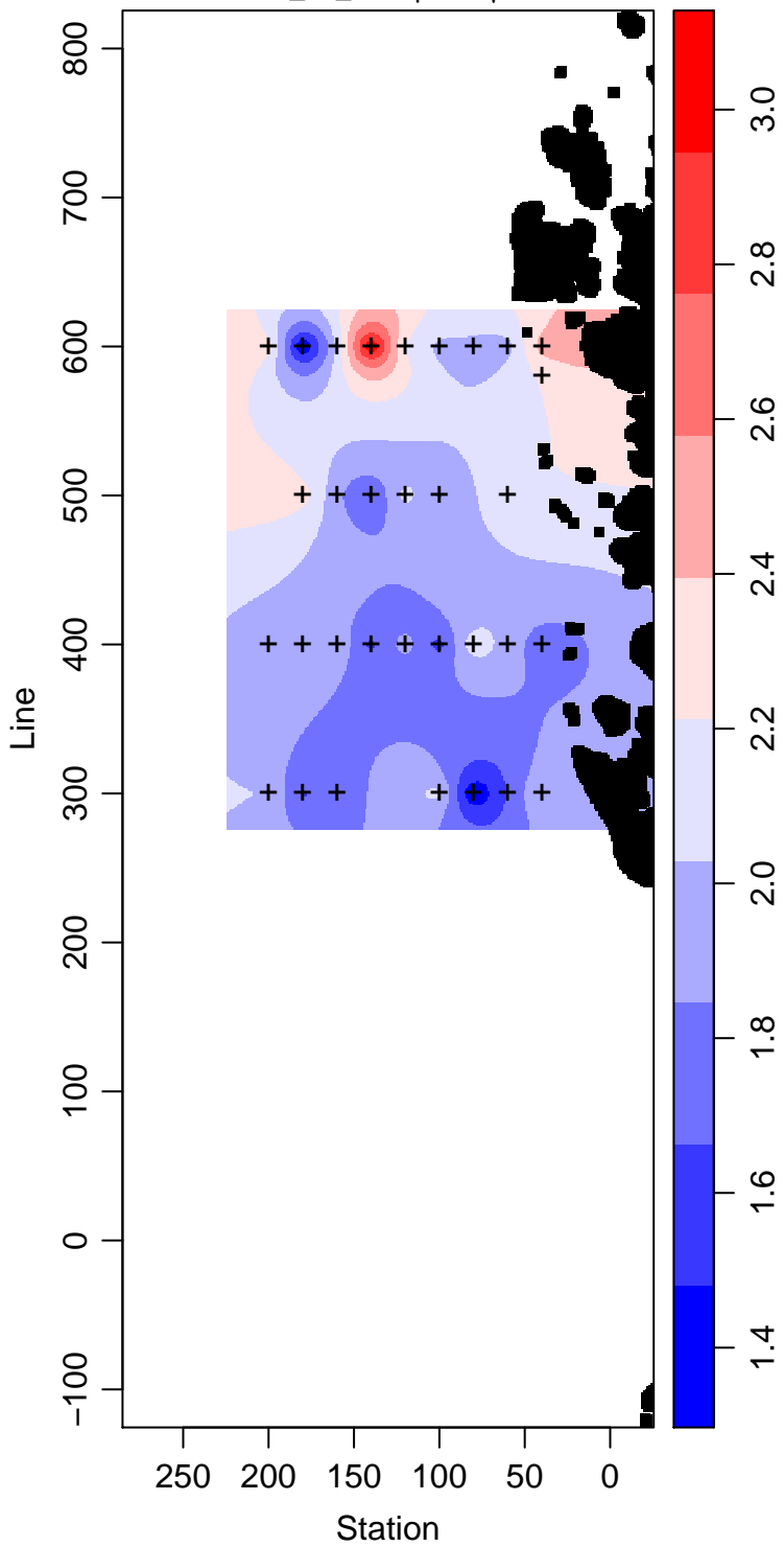
PD94-01_75_Phosphate \mu\text{ mol L}^{-1}
