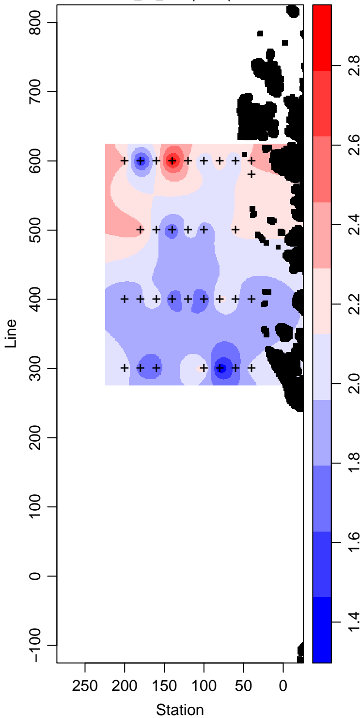
PD94-01_80_Phosphate \mu\text{ mol L}^{-1}
